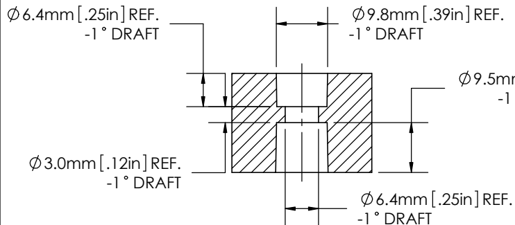
MOUNTING HOLE DETAIL
