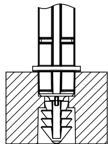
ASSEMBLED VIEW
